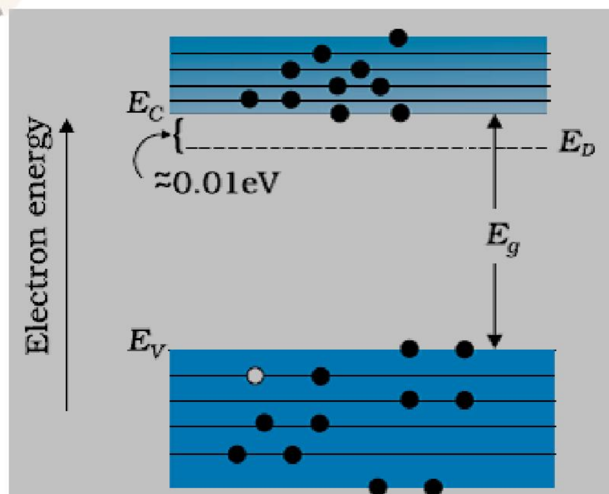
(i) n-type semiconductor at T > 0\text{K}
