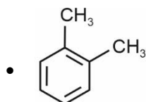
o-xylene
